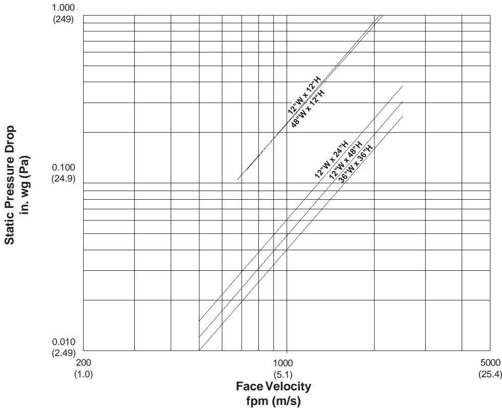
AMCA Figure 5.3
