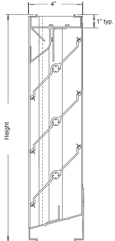
Section View
